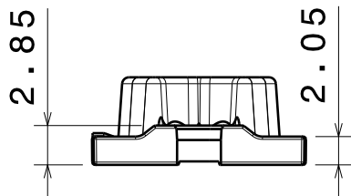
Right view
