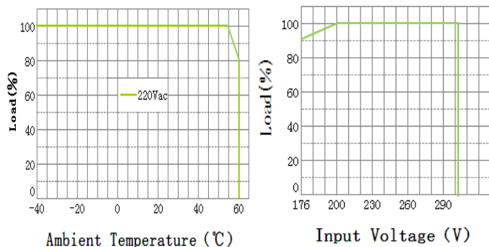
Derating Curve
