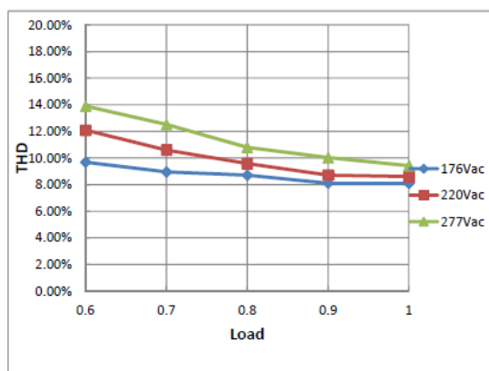
THD Curve
