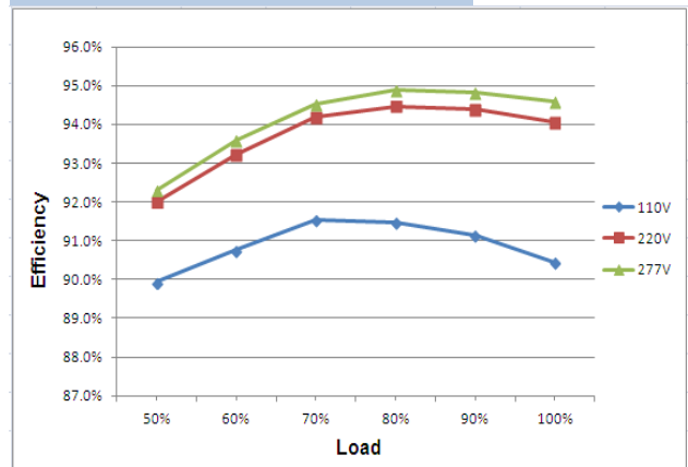
Efficiency VS. Load Curve
