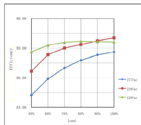
Efficiency VS. Load Curve(Model:700mA)
