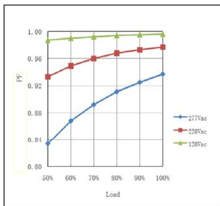
Power Factor VS. Load Curve(Model:700mA)
