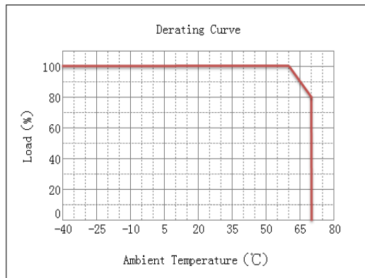
Derating Curve
