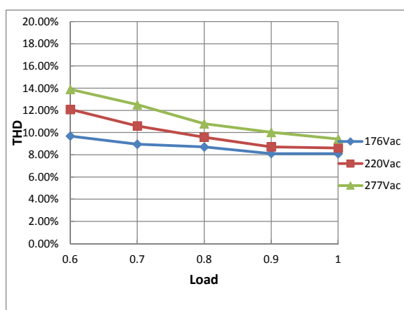
THD Curve
