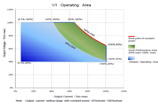
V/I Curve
