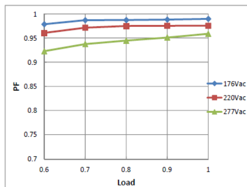
Power Factor Curve
