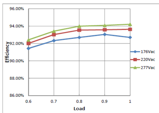
Efficiency VS. Load Curve (Model 850mA)
