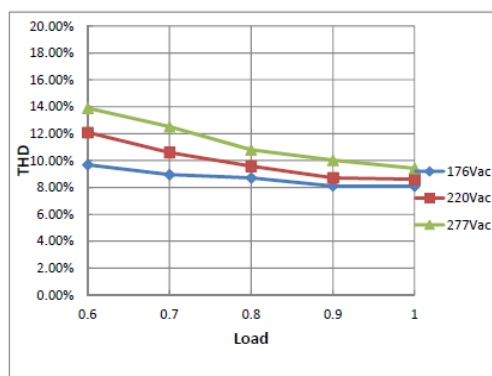
THD Curve
