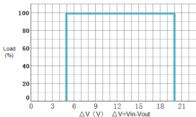
ΔV Curve
