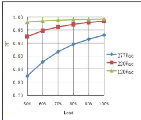
Power Factor VS. Load Curve(Model:700mA)
