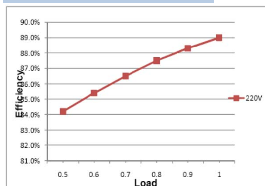
Efficiency VS. Load Curve(Ref. 700mA)
