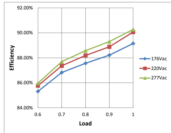
Efficiency VS. Load Curve (ME075M105AQ_CP)
