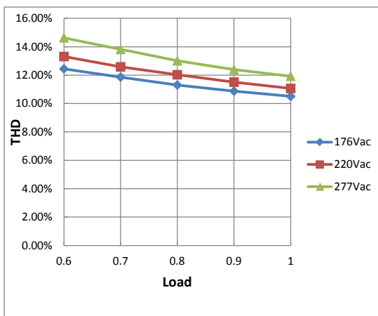
THD Curve
