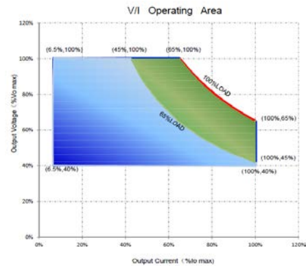
V/I Curve
