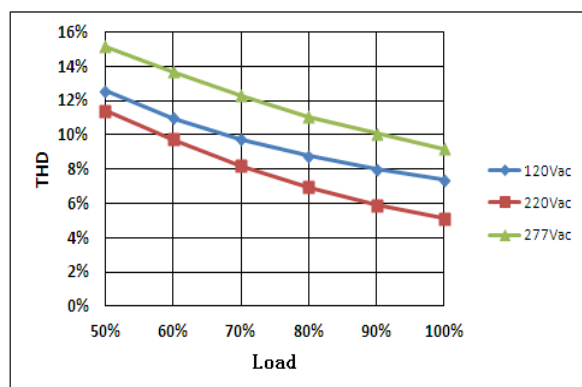
THD Curve
