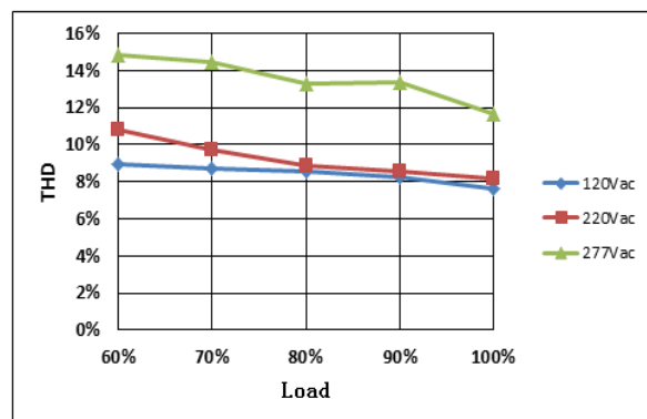
THD VS. Load Curve (900mA)
