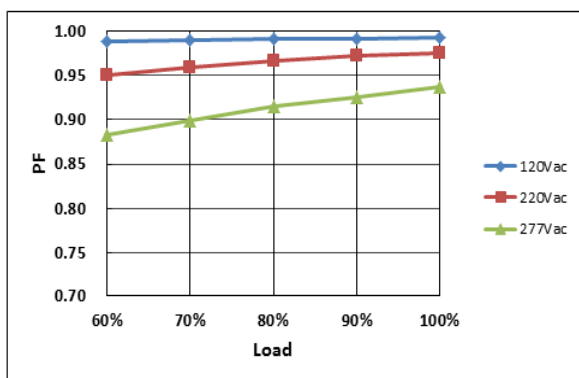
Power Factor VS. Load Curve (900mA)
