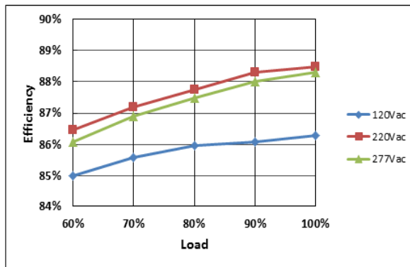
Efficiency VS. Load Curve (900mA)
