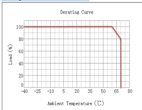
Derating Curve
