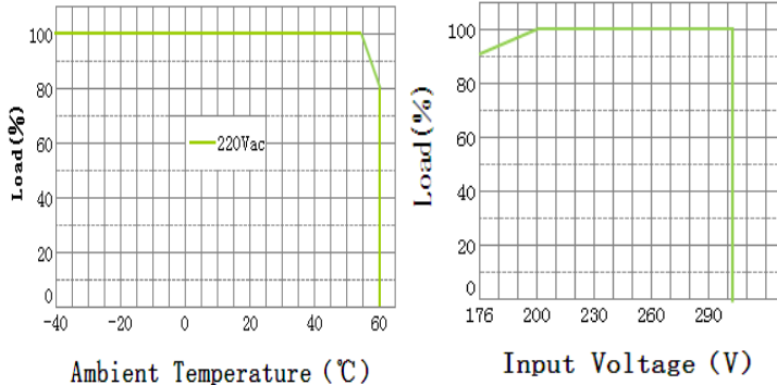
Derating Curve
