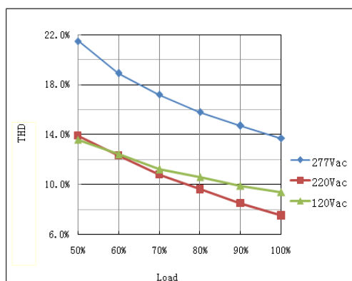
THD Curve
