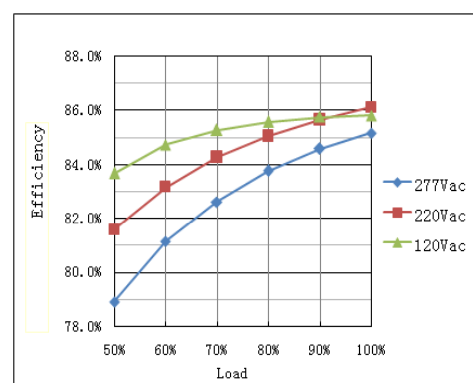
Efficiency VS. Load Curve
