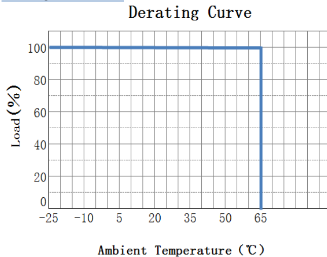
Derating Curve
