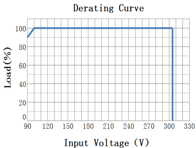
Derating Curve
