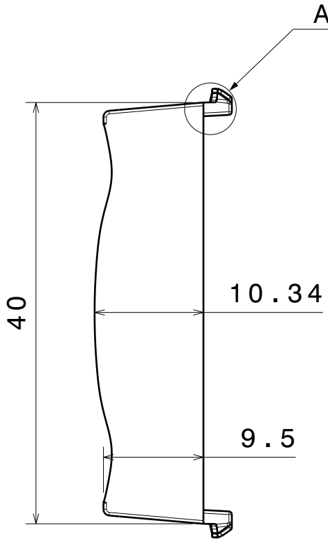
GENERAL MOULDING TOLERANCES
