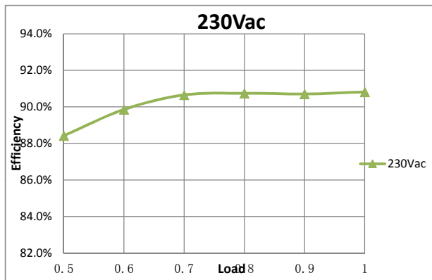
Efficiency VS. Load Curve (MU100P200AQ_0-10V)
