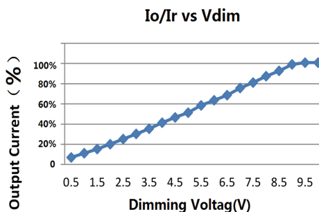
Dimming Curve
