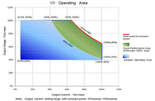
V/I Curve
