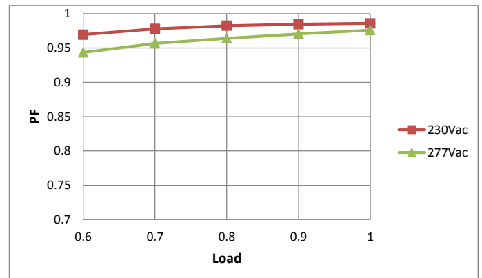
Power Factor Curve
