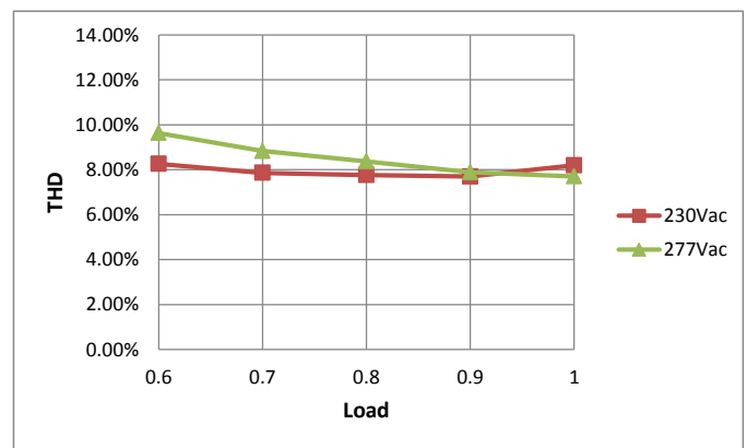
THD Curve
