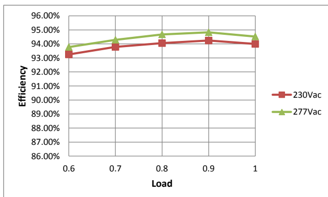
Efficiency VS. Load Curve (Io=1400mA)
