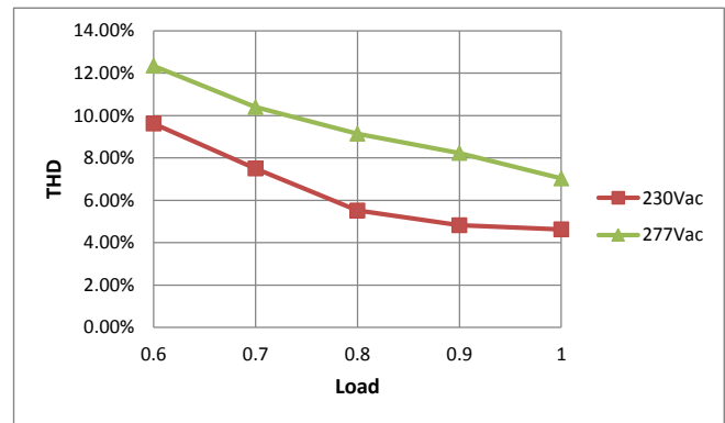
THD Curve
