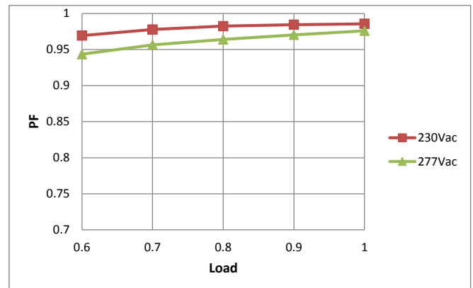
Power Factor Curve
