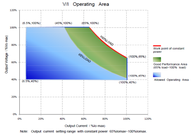
V/I Curve
