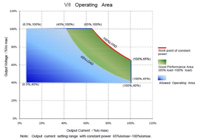
V/I Curve
