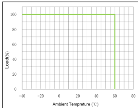
Derating Curve
