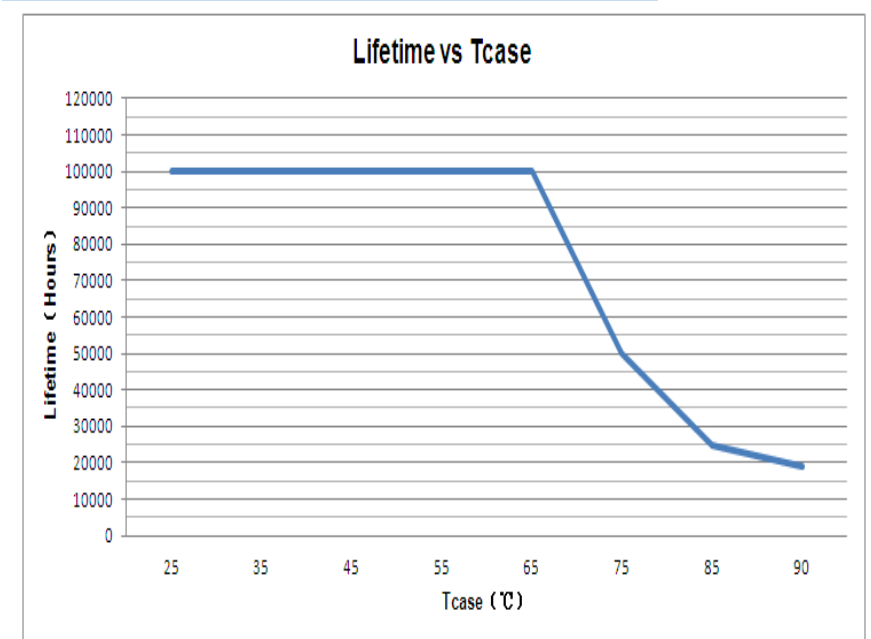
Life Time VS. Tcase (Ref.)
