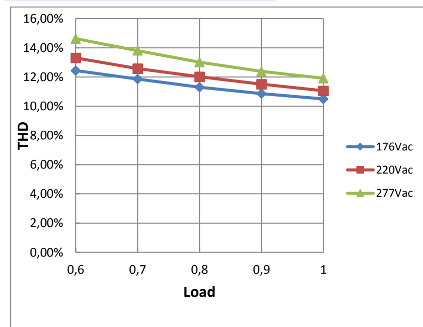
THD Curve
