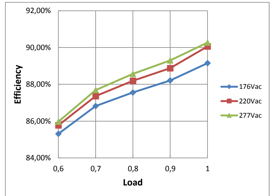
Efficiency VS. Load Curve
