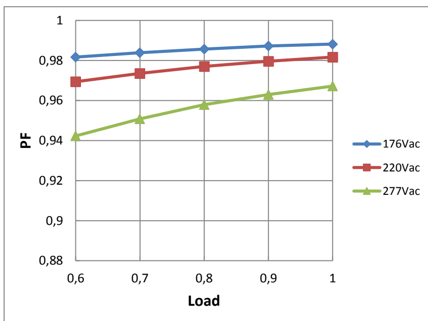
Power Factor VS. Load Curve
