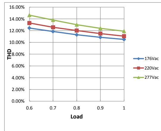
THD Curve
