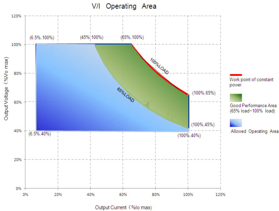
V/I Curve
