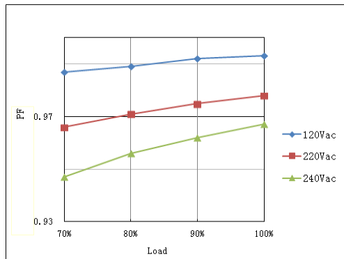
Power Factor VS. Load Curve
