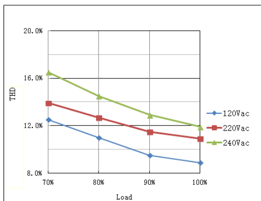
THD Curve
