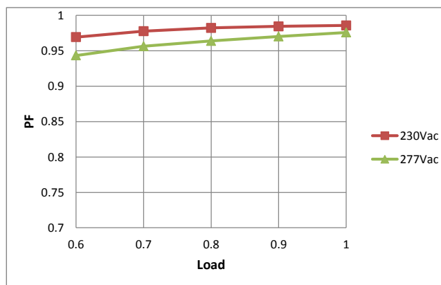
Power Factor Curve
