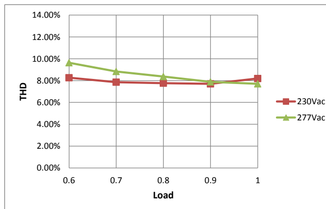
THD Curve
