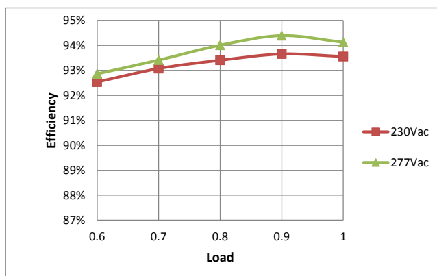
Efficiency VS. Load Curve (Io=4000mA)
