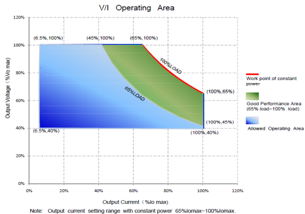
V/I Curve
