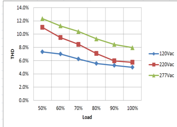
THD Curve
