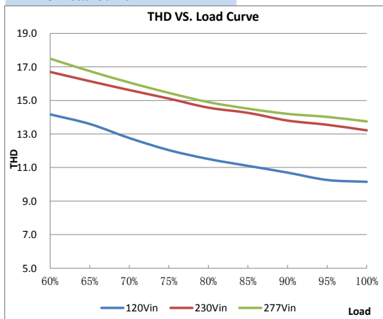
THD VS. Load Curve
