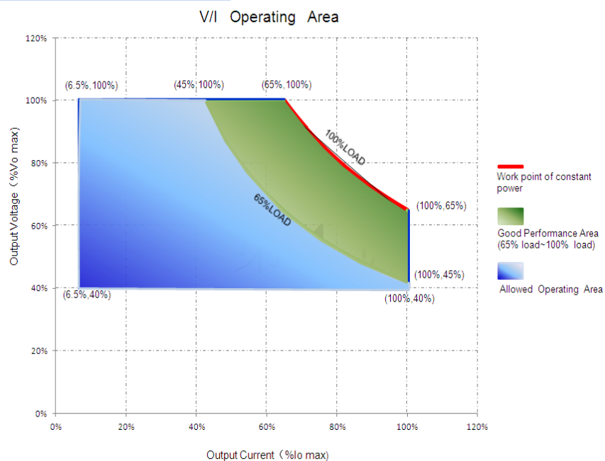
V/I Curve
