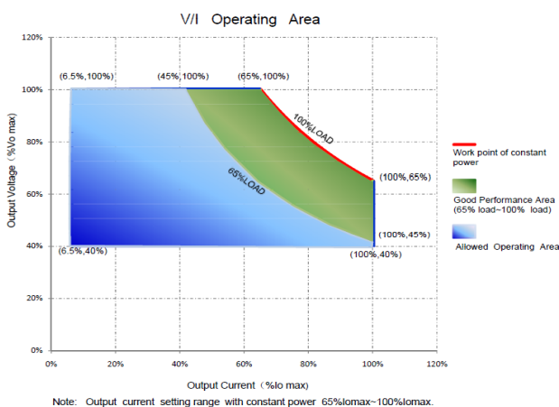
V/I Curve
