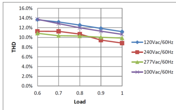
THD Curve
