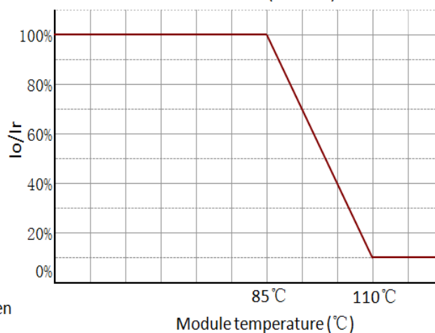
Io/Ir(%) vs Module temperature using NCP18XH103F03RB (Murata)
