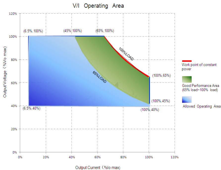
V/I Curve
