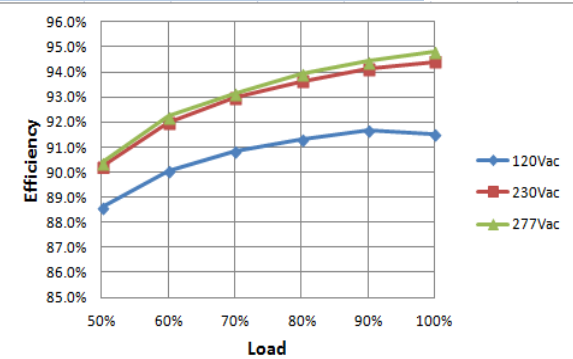
Efficiency VS. Load Curve (1300mA for Ref.)
