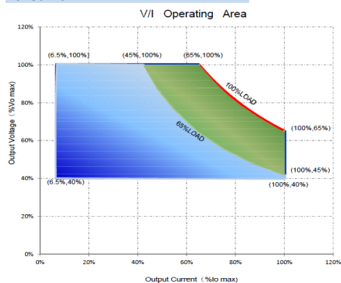
V/I Curve
