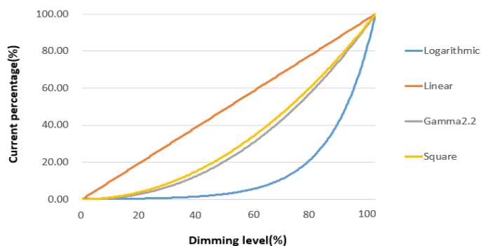
▪ Dimming Curve
