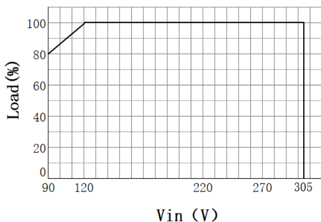
▪ Derating Curve ( I_o > 700mA \cdot 4CH )
