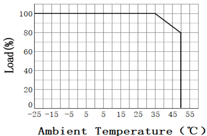
▪ Derating Curve ( I_o > 700mA \cdot 4CH )
