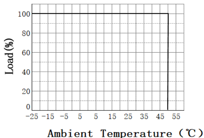
▪ Derating Curve ( I_o \leq 700mA \cdot 4CH )
