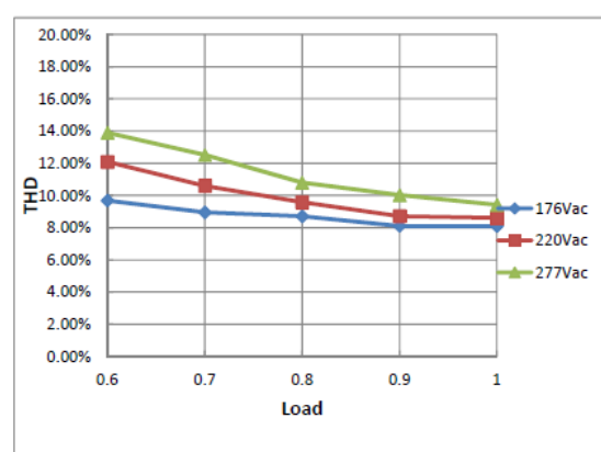
THD Curve
