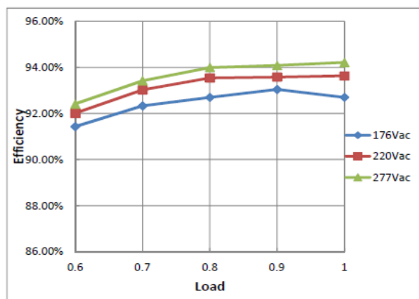
Efficiency VS. Load Curve (Model 850mA)
