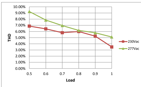
THD Curve
