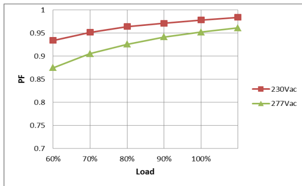
Power Factor VS. Load Curve
