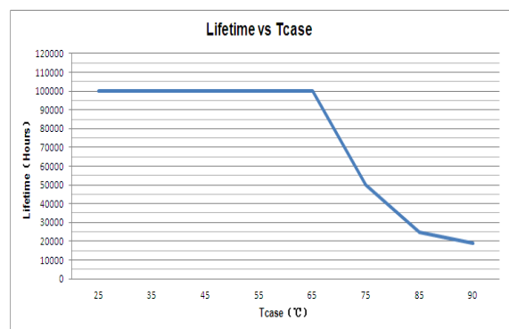
Life Time VS. Tcase (Ref.)
