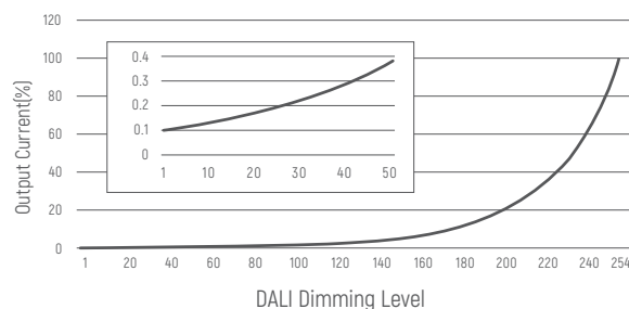
Dimming Curve
