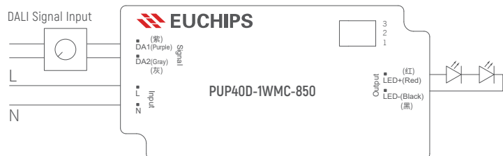
Wring Diagram
