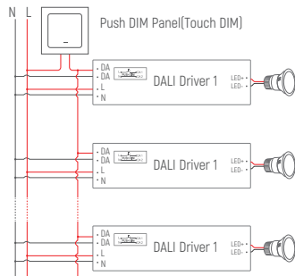
Touch DIM(Push DIM) Diagram
