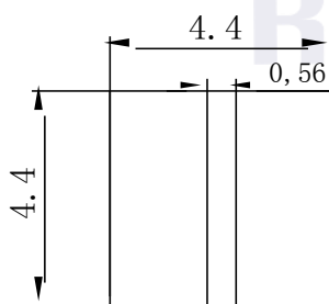
Fig.1-5 Soldering patterns 推荐焊盘
