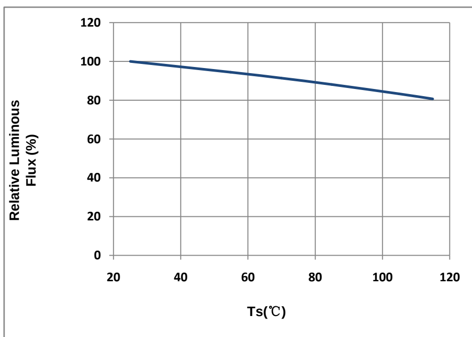
Fig 1-11 Solder Temperature Vs Relative Intensity 管脚温度与相对光强特性曲线
