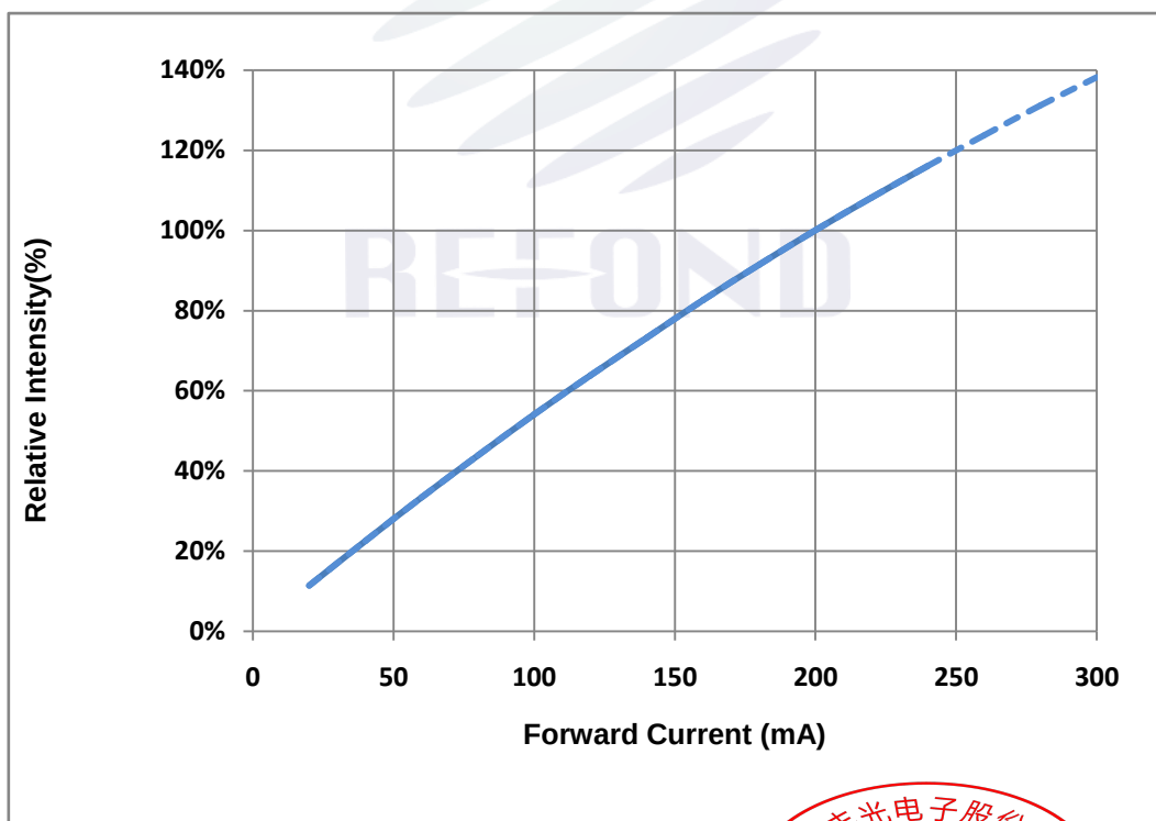
Fig 1-10 Forward Current Vs. Relative Intensity 正向电流与相对光强特性曲线
