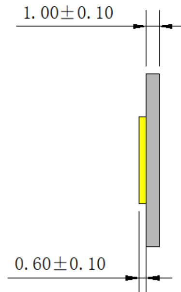
Fig.1-2 Side view 侧面视图
