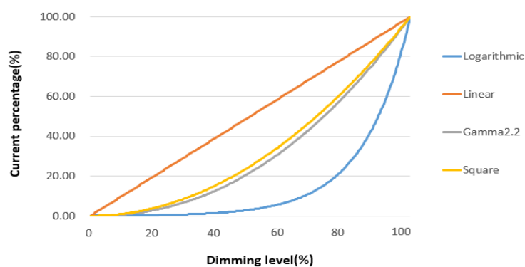
■ Dimming Curve
