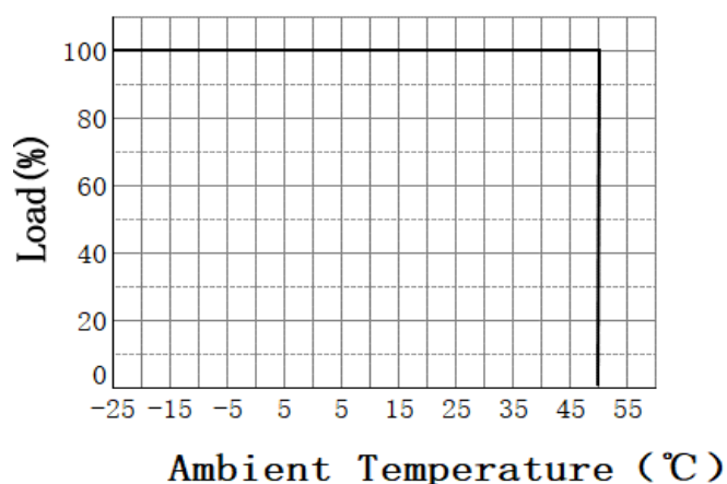
▪ Derating Curve ( I_o \leq 700\text{mA} \times 4\text{CH} )
