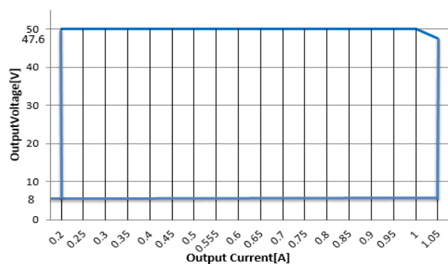
▪ V/I Curve(1CH for ref)
