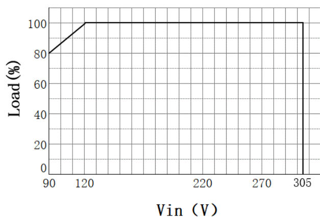
▪ Derating Curve ( I_o > 700\text{mA} \times 4\text{CH} )
