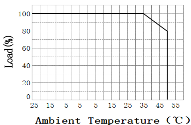
▪ Derating Curve ( I_o > 700\text{mA} \times 4\text{CH} )
