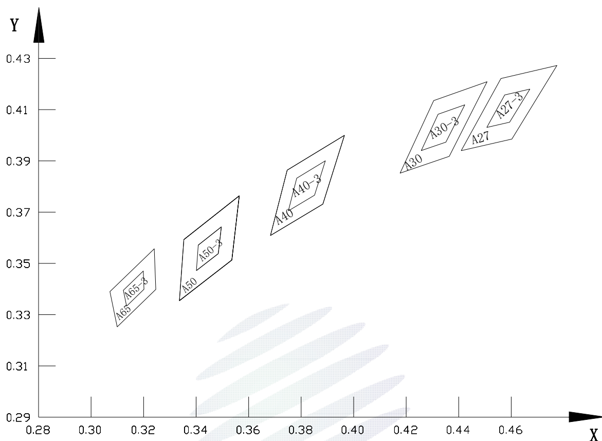
Fig 1-6 The C.I.E Chromaticity Diagram CIE色度
