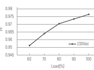
PF vs 负载
