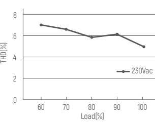
THD vs 负载
