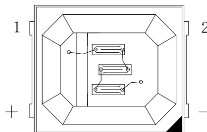
Fig.1-6 Chip configuration 芯片排布
