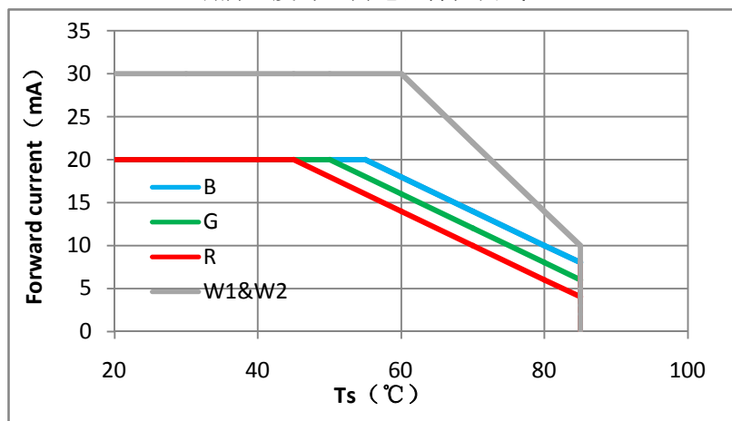
Fig.7-Pin Temperature Vs. Forward Current
