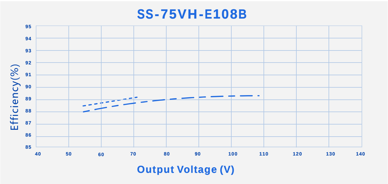
Efficiency Vs. O/P Voltage (Vin=120Vac)
