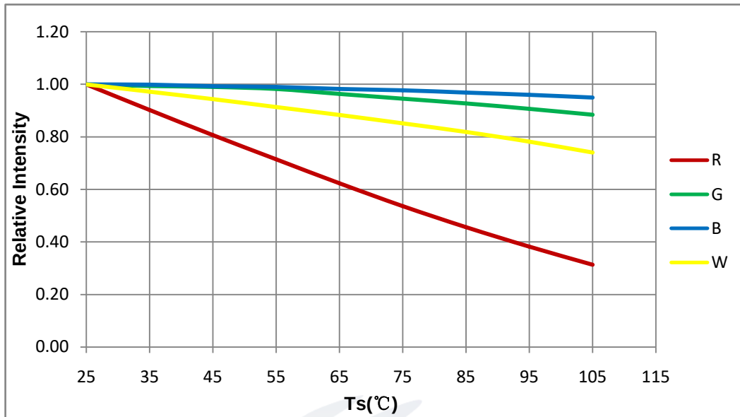
Fig.1-8 Temperature Vs. Relative Intensity 引脚温度与相对光强特性曲线
