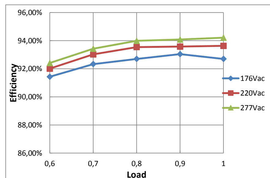
Efficiency VS. Load Curve
