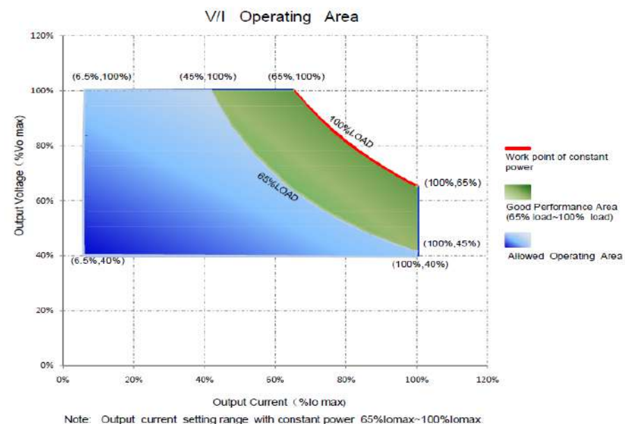
V/I Curve
