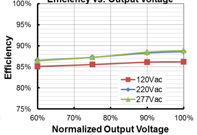
EAM-075S210SB(I o =2100mA) Efficiency vs. Output Voltage
