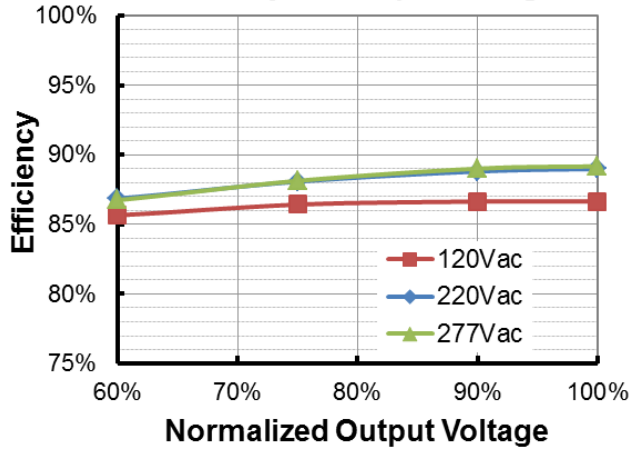
EAM-075S210SB(I o =1400mA) Efficiency vs. Output Voltage
