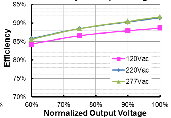
EAM-100S150SB(I o =1500mA) Efficiency vs. Output Voltage
