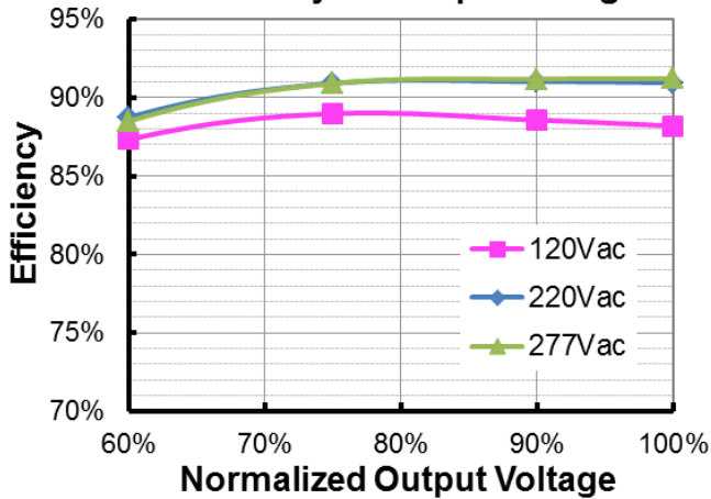
EAM-100S150SB(I o =1050mA) Efficiency vs. Output Voltage
