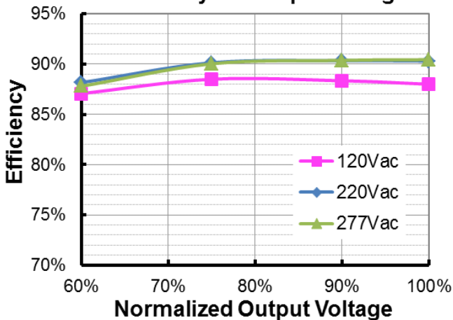
EAM-100S280SB(I o =1750mA) Efficiency vs. Output Voltage
