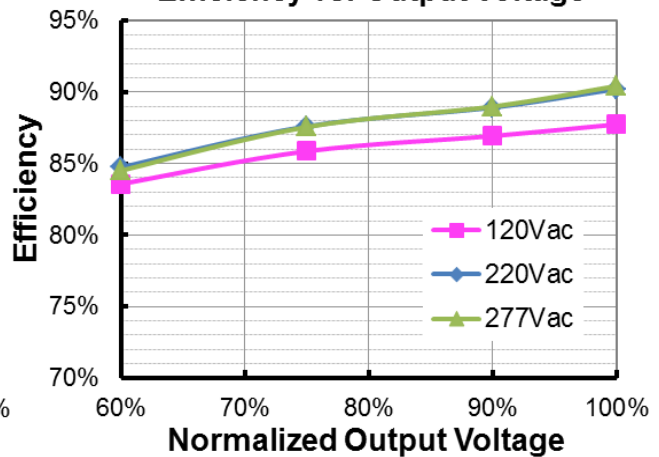
EAM-100S280SB(I o =2800mA) Efficiency vs. Output Voltage
