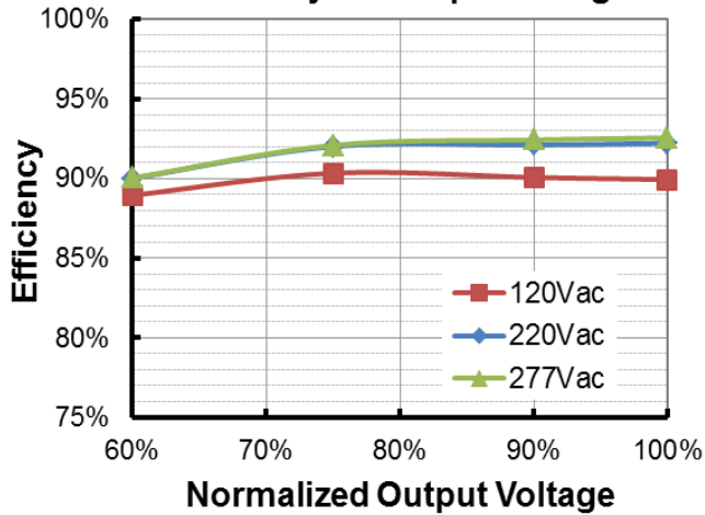
EAM-150S150SB(I o =1050mA) Efficiency vs. Output Voltage
