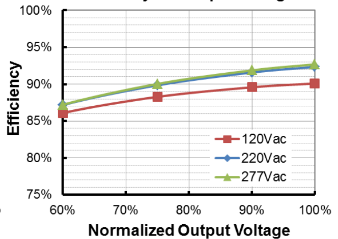
EAM-150S150SB(I o =1500mA) Efficiency vs. Output Voltage
