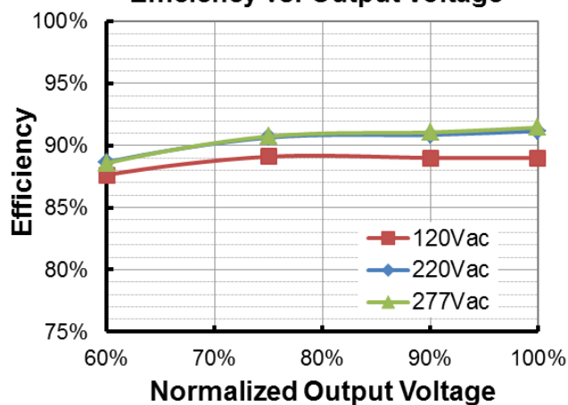
EAM-150S420SB(I o =2800mA) Efficiency vs. Output Voltage
