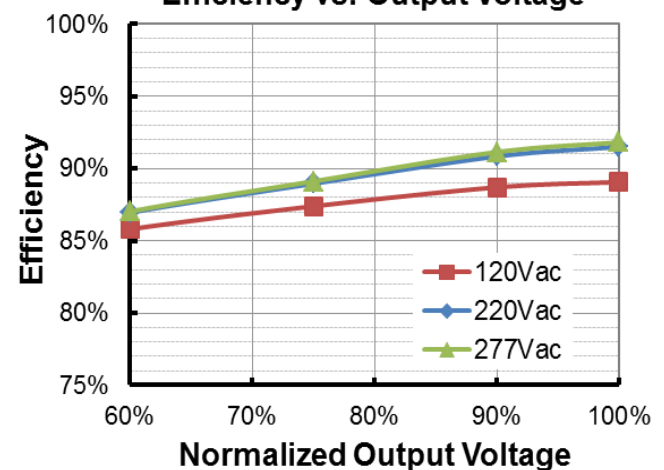
EAM-150S420SB(I o =4200mA) Efficiency vs. Output Voltage
