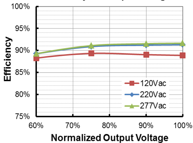
EAM-150S210SB(I o =1400mA) Efficiency vs. Output Voltage
