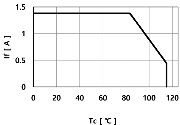
Derating Curve (LC019D)
