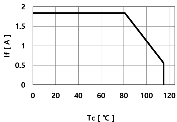
Derating Curve (LC026D)
