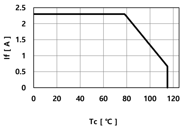
Derating Curve (LC033D)
