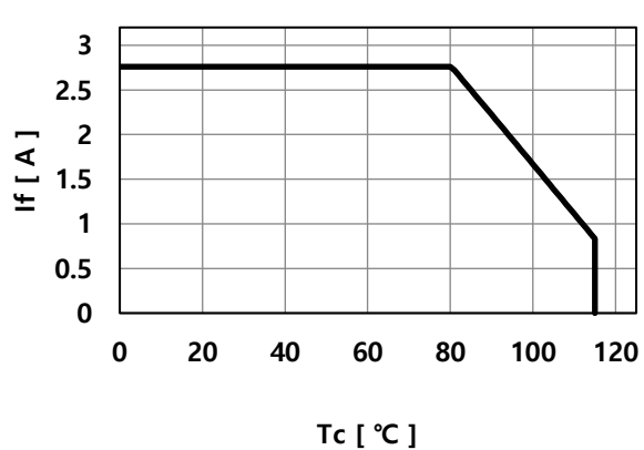
Derating Curve (LC040D)
