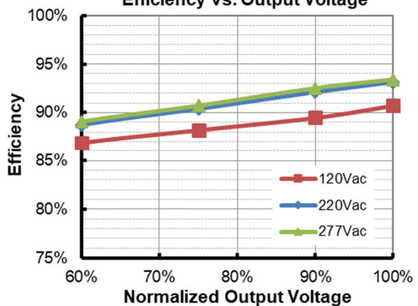
EUM-240S210Ex ( I_o=3500mA ) Efficiency vs. Output Voltage
