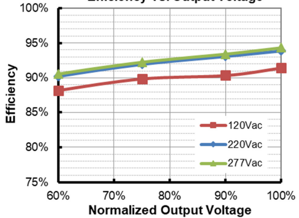
EUM-240S105Ex ( I_o=1050mA ) Efficiency vs. Output Voltage
