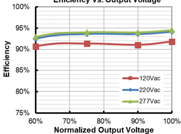
EUM-240S350Ex ( I_o=2150mA ) Efficiency vs. Output Voltage
