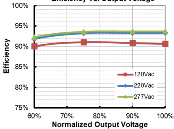
EUM-240S150Ex ( I_o=1050mA ) Efficiency vs. Output Voltage
