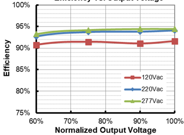
EUM-240S105Ex ( I_o=700mA ) Efficiency vs. Output Voltage
