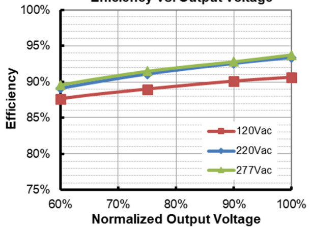
EUM-240S150Ex ( I_o=1500mA ) Efficiency vs. Output Voltage
